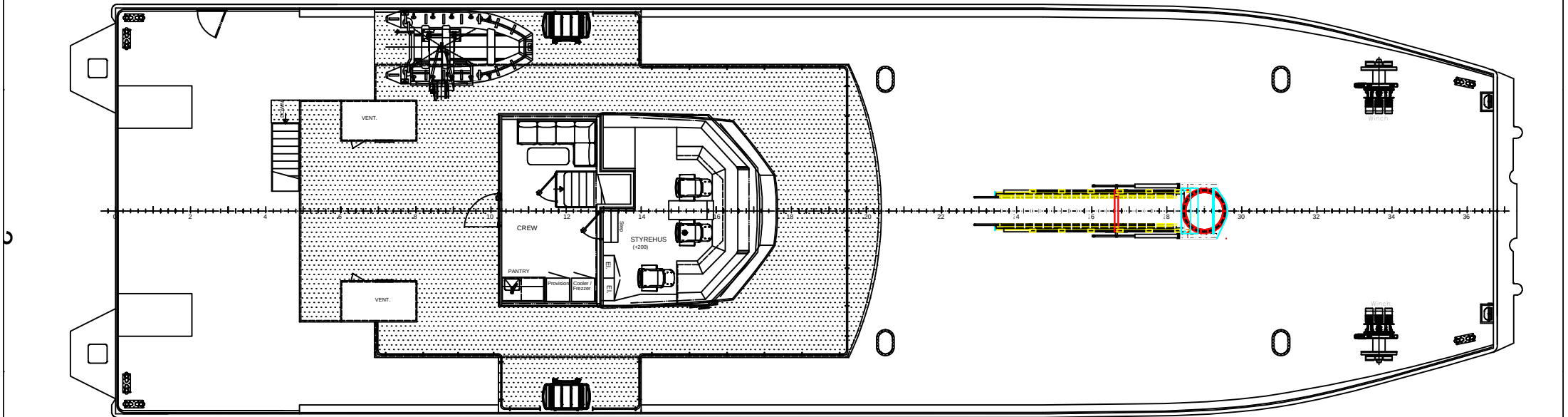
PLAN TOP DECK
